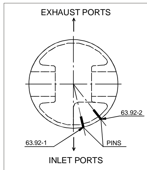
VIEW FROM TOP
