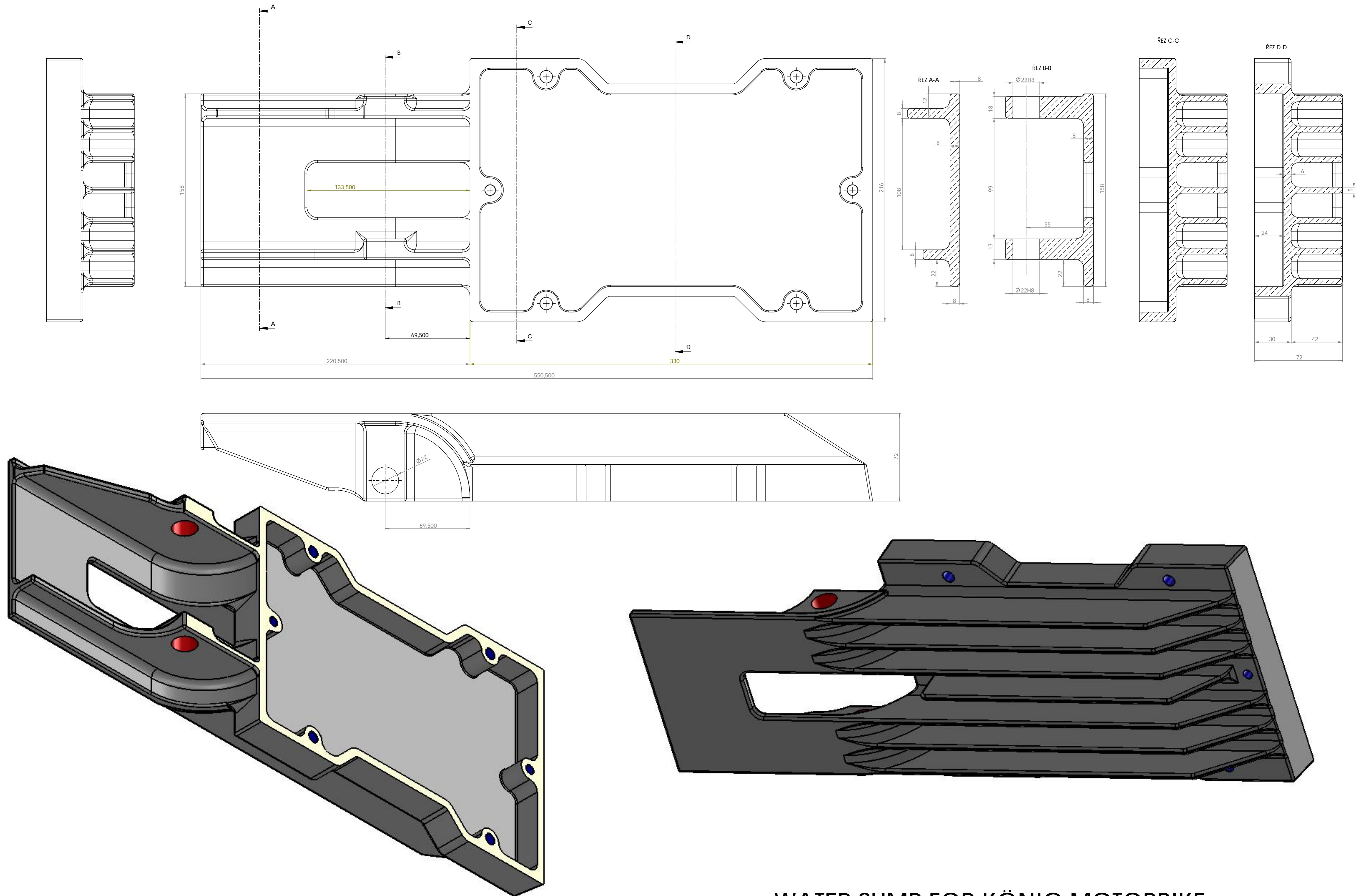
WATER SUMP FOR KÖNIG MOTORBIKE CNC MACHINED FROM SOLID ALUMINIUM BLOCK
